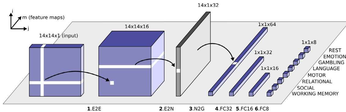
FIGURE 1 Schematic overview of the modified convolutional neural network architecture used to classify the eight different network configurations (seven tasks and one resting state; Kawahara et al., 2017). Each block represents the input/output of a numbered filter layer. The third dimension ( m ) represents the result of convolving the input with m different filters (feature maps). First, an interaction matrix composed of the interactions of 14 networks (based on synchrony or metastability) is entered as input. This is convolved with an edge-to-edge (1, E2E) filter which weights the edges associated with adjacent brain networks in topological space. The output from this layer is then convolved with an edge-to-node (2, E2N) filter which assigns each network a weighted sum of its edges. Next, a node-to-graph (3, N2G) layer outputs a single response based on all the weighted nodes. Finally, the number of features is reduced to eight output classifications through a series of fully connected (4/5/6, FC) layers
